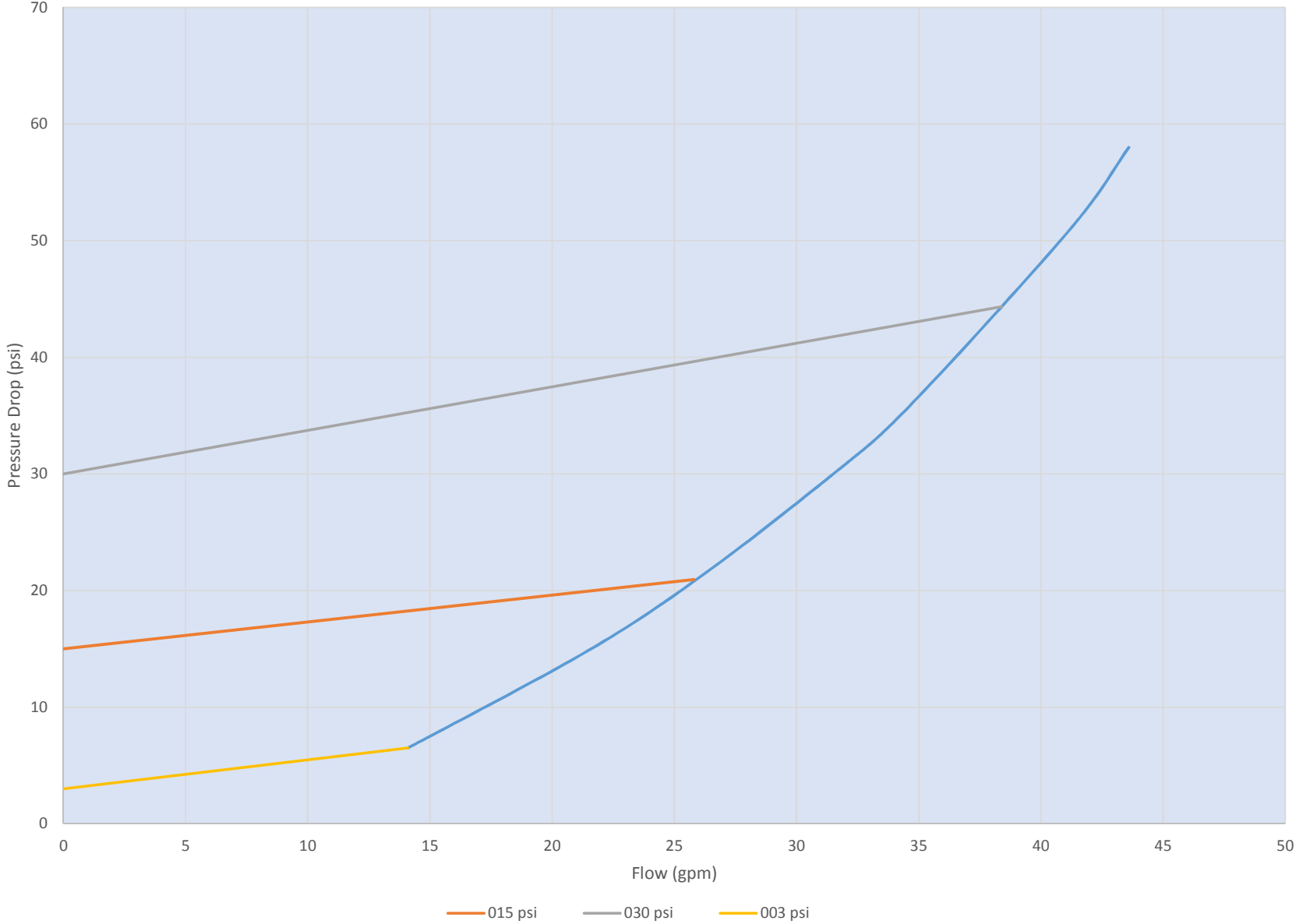
ICT-B-16 Pressure Drop versus Flow (ISO 68 Oil, 100F )
