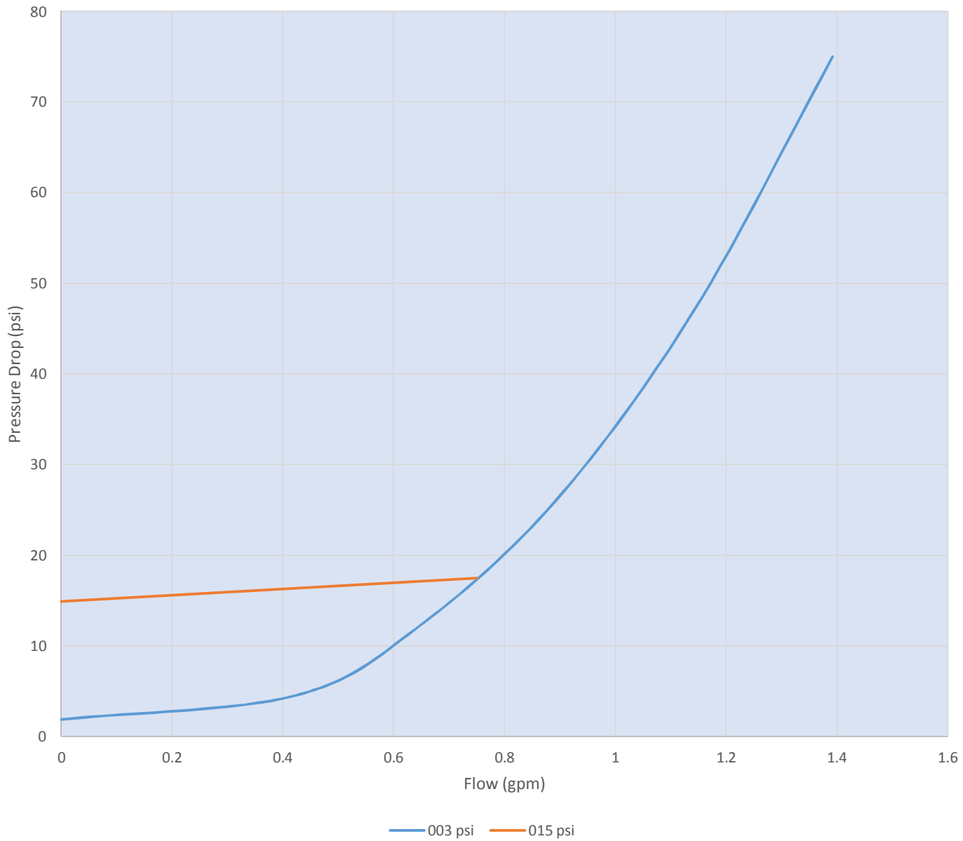
ICT-B-02 Pressure Drop versus Flow (ISO 68 Oil, T=100F )
