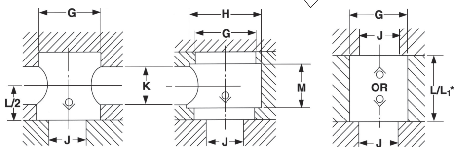
TEE BRANCH RIGHT ANGLE STRAIGHT THRU (COMBINATIONS OF THESE CAVITIES CAN BE USED)
